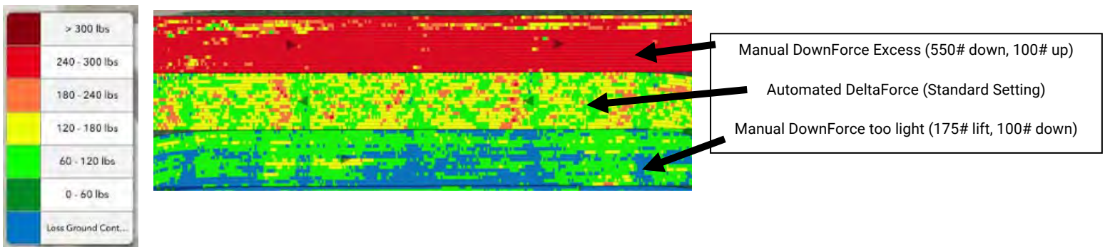
Weight carried on gauge wheels.
