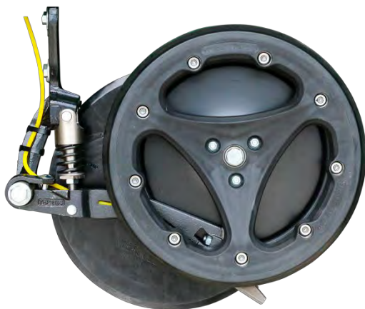
Figure 1. Conceal Knife Design within Gauge Wheel
