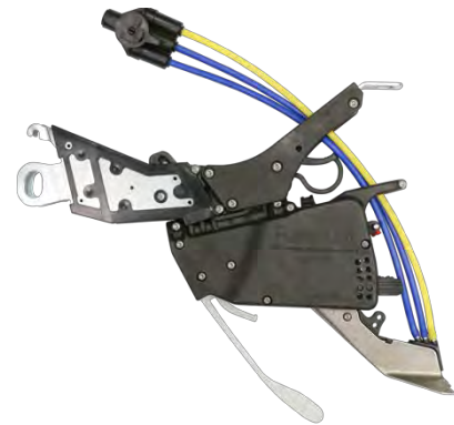
Figure 2: FurrowJet Dual-Band Wings Fracturing Side-Walls
