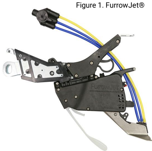
Figure 1. FurrowJet®
