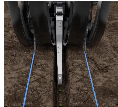
Figure 1. Conceal® placement 3” away from seed furrow and 1.5” deep
