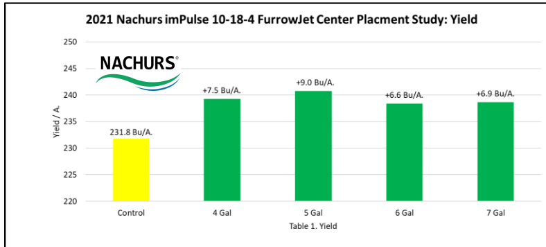
Figure 1. FurrowJet® Placement
