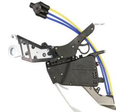
Figures 2-3: FurrowJet® Dual-Band Wings Fracturing Sidewalls
