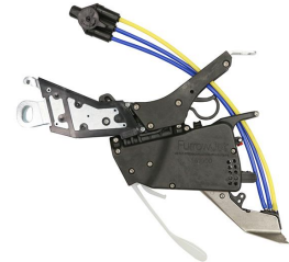
Figure 1. FurrowJet® Placement
