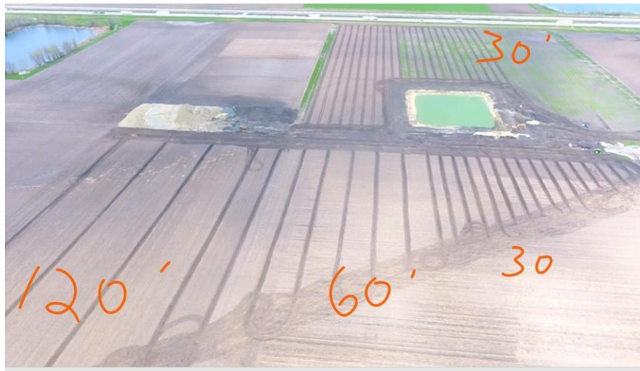
Figure 5. 30', 60', 120' Tile Patterns
