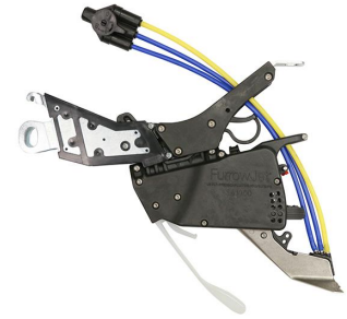
Figure 1. FurrowJet® Placement
